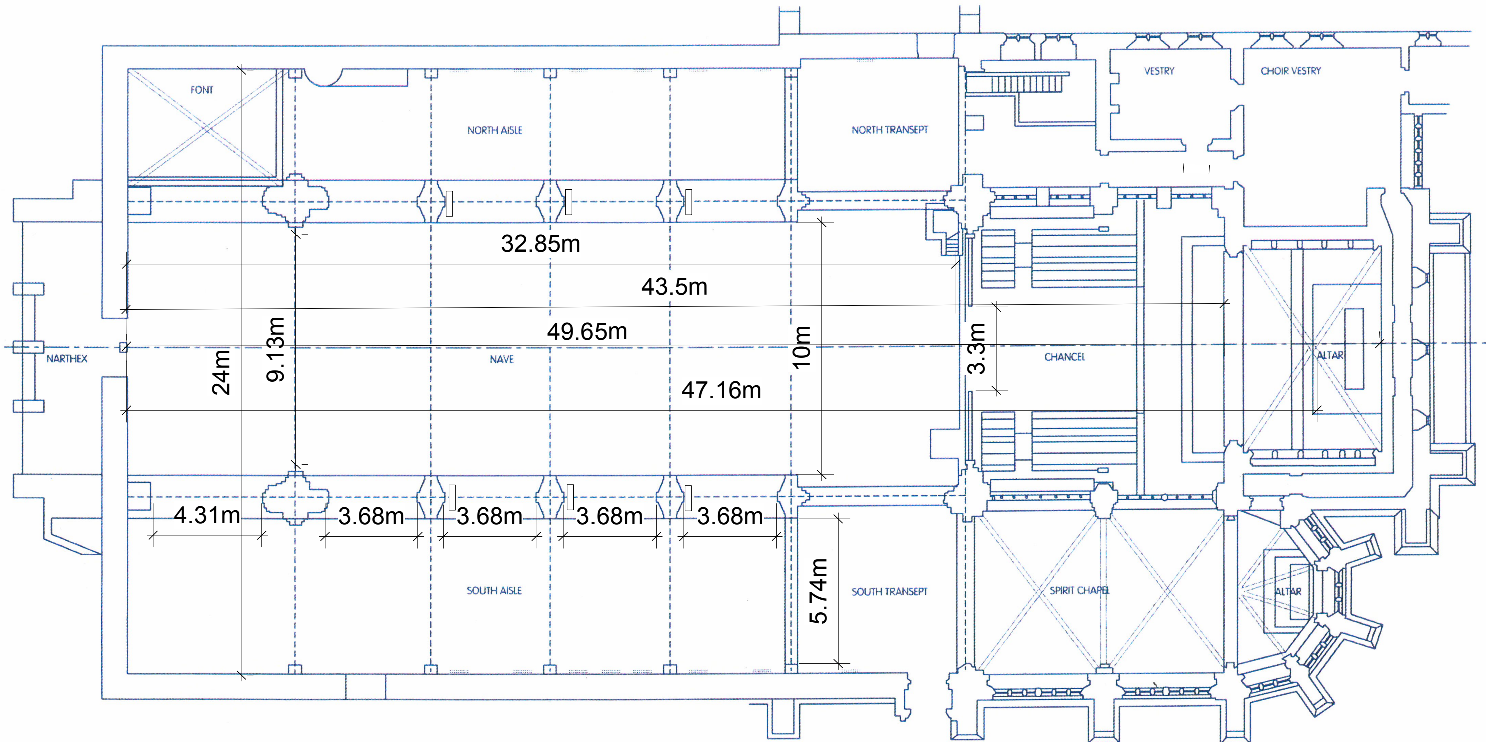
All Saints Church, Eton Road, Hove. Scale: 1:150
